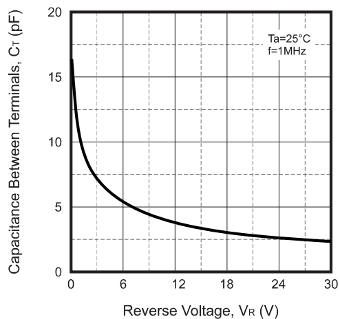
Fig.3 - Capacitance Characteristics Per Diode
